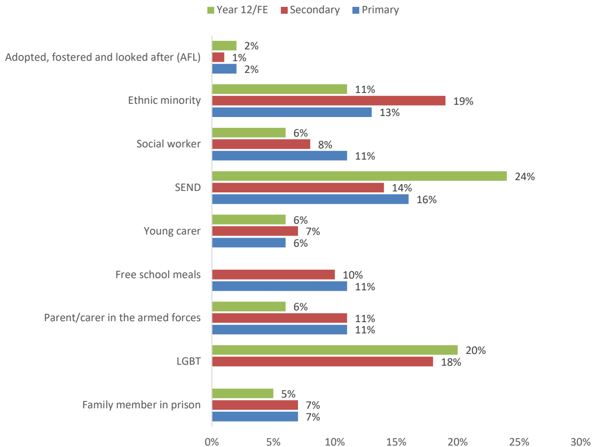
Figure 1: Vulnerable groups
